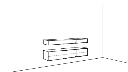
combination VE04 h18 x w216 x d36 h36 x w216 x d36
