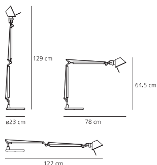
Tolomeo Tolomeo Led Tolomeo Led MWL
