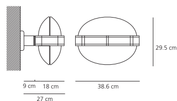
Alcesti parete FLUO 2x26W (G24 d-3) – TC-D
