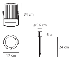
Metamorfosi kit outdoor HALO 3x150W (B 15d) – ES with or without remote control
