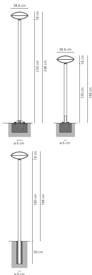
Alcesti terra FLUO 2x26W (G24 d-3) – TC-D
