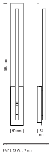
WLS 96 Wall fixture Design: Thomas Schultz, 1996.
