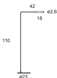
Cod. 945 Flo Floor
