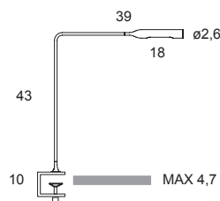
Cod. 955 Flo Clamp
