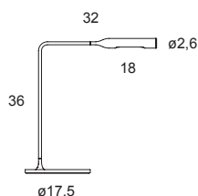
Cod. 950 Flo Bedside
